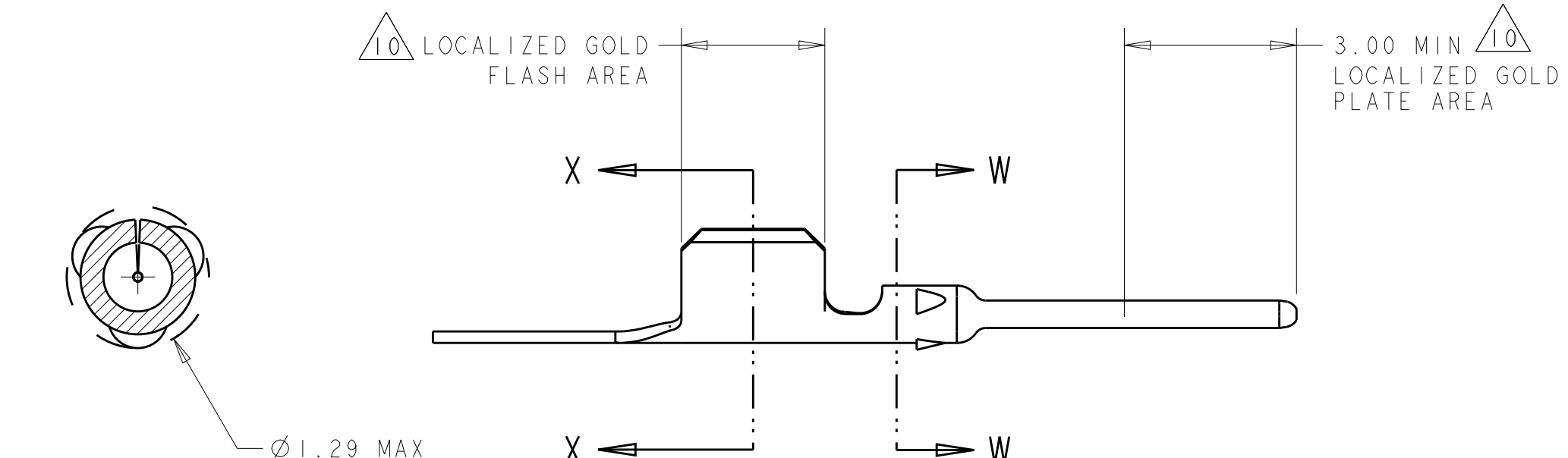
SECTION W-W SCALE 20:1
