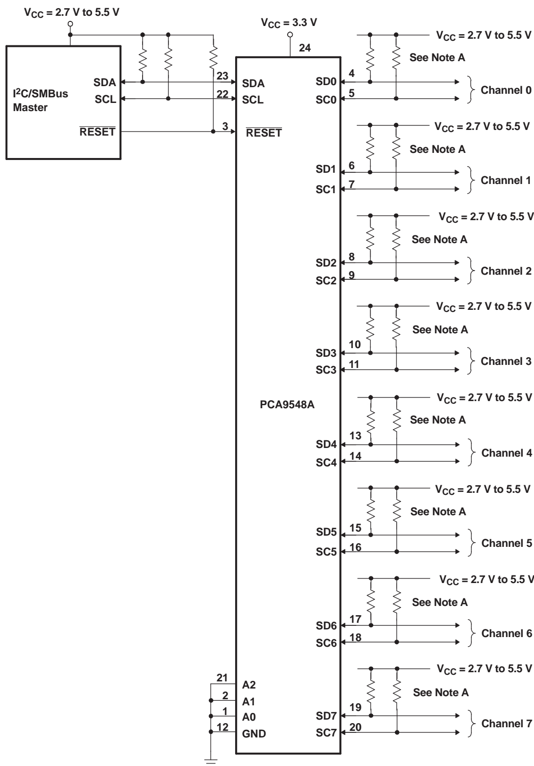
Figure 11. Typical Application
