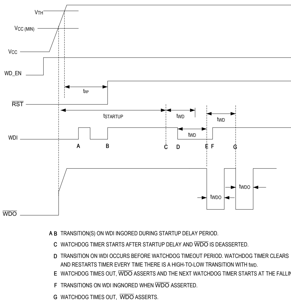
Figure 1. Watchdog Timing Characteristics with \text{WD\_EN} Active During Power-Up
