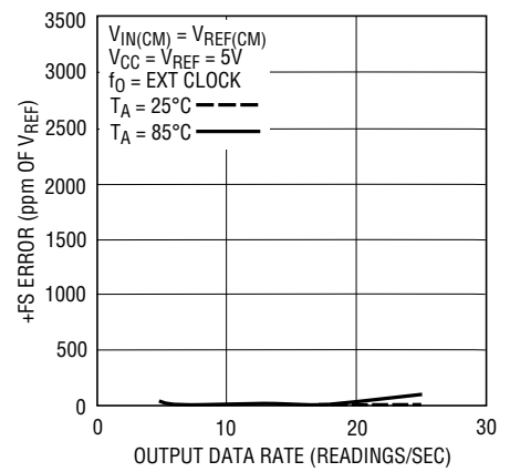
Figure 32. +FS Error vs Output Data Rate and Temperature
