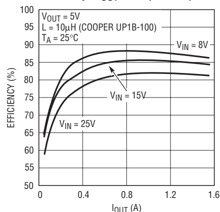
Efficiency, V_{OUT} = 5V (LT3506)
