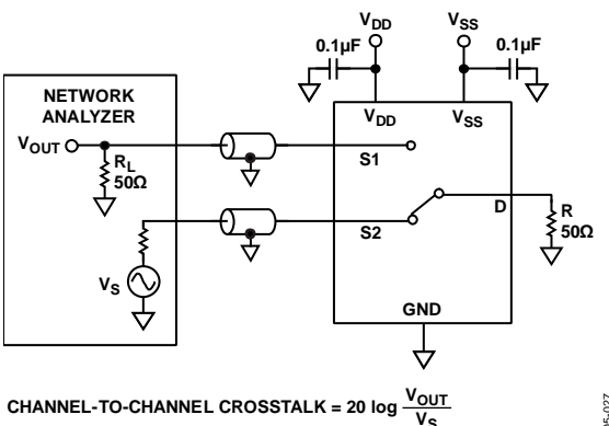
Figure 29. Channel-to-Channel Crosstalk
