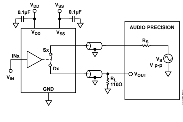
Figure 31. THD + Noise
