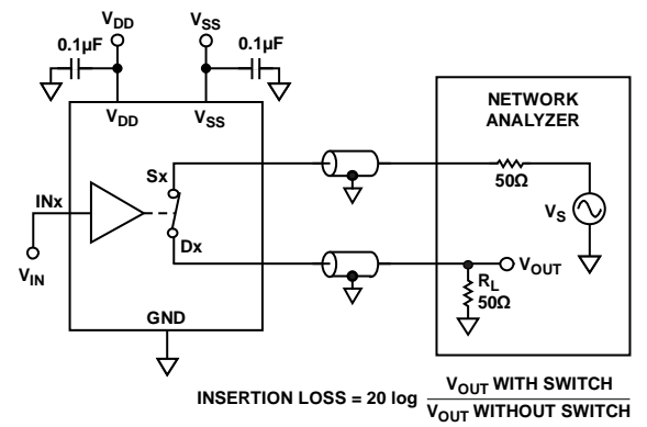
Figure 30. Bandwidth
