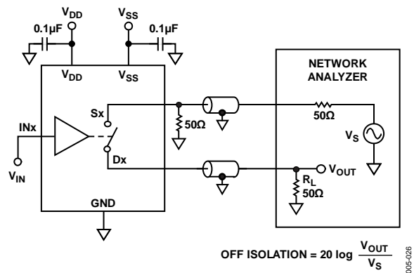
Figure 28. Off Isolation
