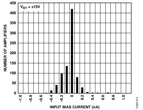
Figure 31. Input Bias Current Distribution, V_{SY} = \pm 15V
