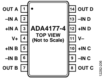
Figure 7. 14-Lead TSSOP Pin Configuration, ADA4177-4
