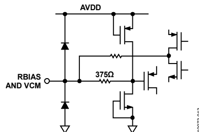
Figure 51. Equivalent RBIAS and VCM Circuit
