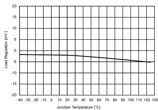
Figure 7. Load regulation vs. temperature ( V_{OUT} = 3.0\ \text{V} , I_{OUT} = 1\ \text{A} to 10\ \text{mA} )
