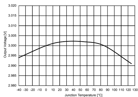
Figure 5. Output voltage vs. temperature ( V_{IN} = 3.0\ \text{V} , I_{OUT} = 1\ \text{A} , normal mode)
