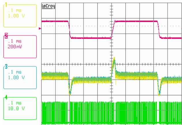
FIGURE 32. VID TOGGling, V_{IN} = 12.6V , I_O = 16.5A , HFM/LFM VID = 1.05V/0.8375V, FDE = DPRSLPVR, Ch1: PMON, Ch2: V_O , Ch3: 40k/100pF FILTERED PMON, Ch4: PHASE
