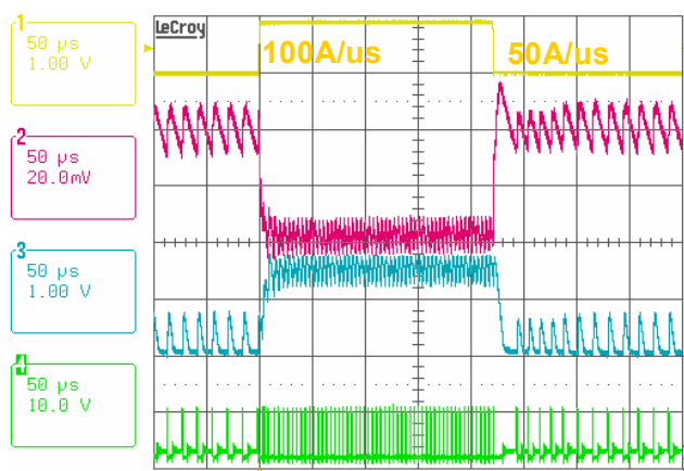
FIGURE 36. LOAD TRANSIENT RESPONSE IN EDEM V_{IN} = 8V , I_O = 2A \leftrightarrow 20A , VID = 1.1V, Ch1: I_O , Ch2: V_O , Ch3: PMON, Ch4: PHASE
