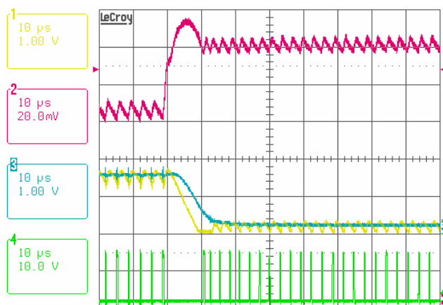
FIGURE 34. LOAD TRANSIENT RESPONSE IN CCM V_{IN} = 12.6V , I_O = 20A \rightarrow 2A (50A/μs), VID = 1.1V, Ch1: PMON, Ch2: V_O , Ch3: 40k/100pF FILTERED PMON, Ch4: PHASE
