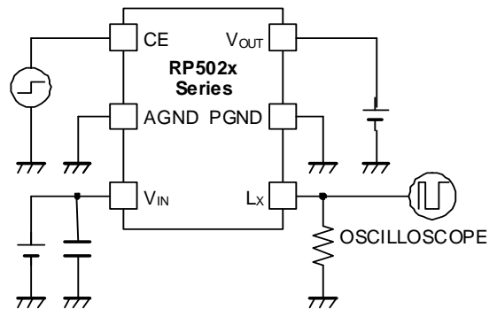
Soft-start Time
