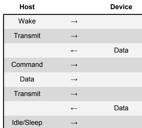
Figure 5-2. Example (Single-Wire)
