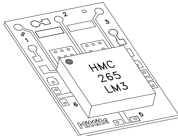
LM3 package mounted to evaluation PCB
