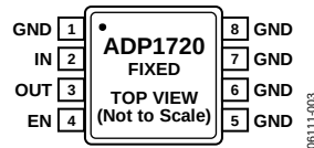
Figure 3. 8-Lead MSOP
