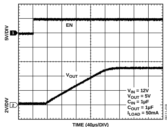
Figure 18. Start-Up Time
