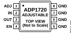
Figure 4. 8-Lead MSOP
