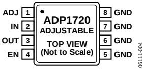
Figure 4. 8-Lead MSOP
