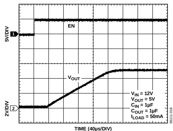
Figure 18. Start-Up Time
