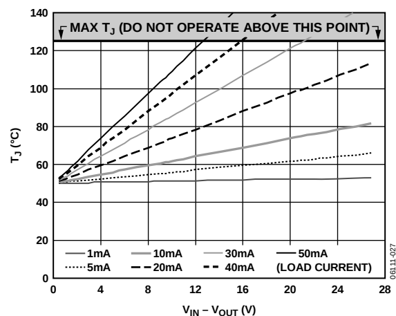
Figure 27. 0 mm 2 of PCB Copper, T_A = 50^\circ\text{C}
