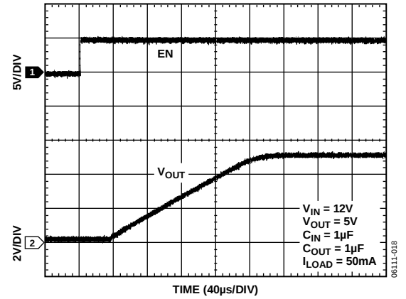
Figure 18. Start-Up Time
