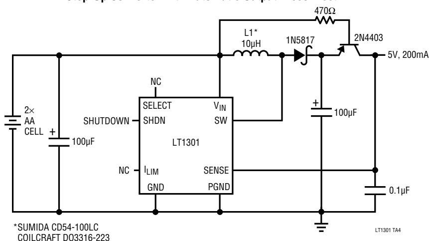
Step-Up Converter with Automatic Output Disconnect
