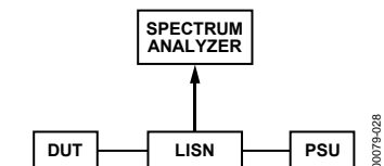
Figure 28. Conducted Emissions Test Setup
