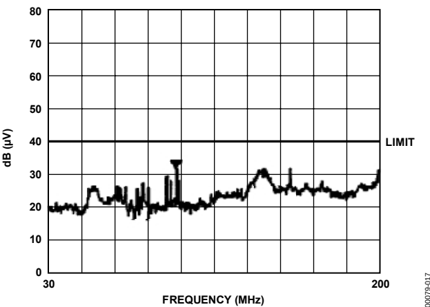
Figure 22. Radiated Emissions
