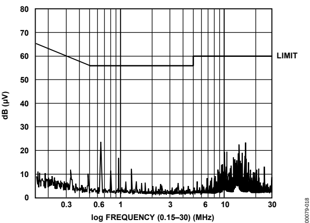
Figure 23. Conducted Emissions
