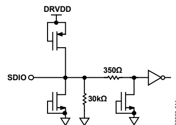
Figure 28. Equivalent SDIO Circuit
