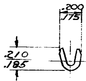
SECT. -A-A
