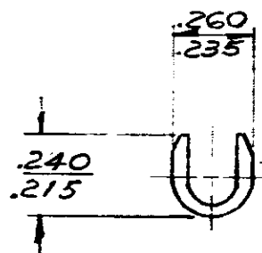
SECT. - B-B
