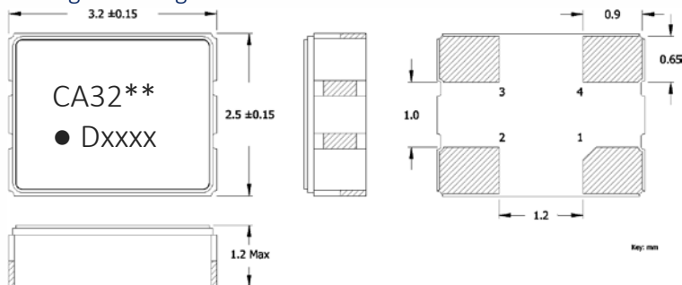
Package Drawing
