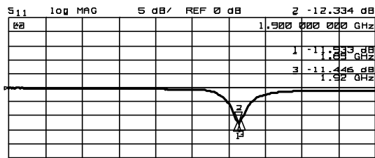
MIXER IN PORT IMPEDANCE
