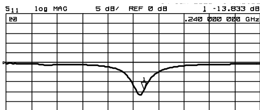
IF OUT PORT IMPEDANCE
