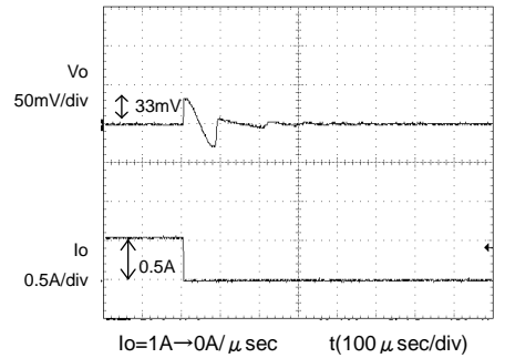
Fig.6 Transient Response (0.5→0A) Co=22 \mu F, Cfb=1000pF
