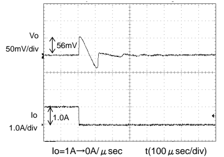
Fig.12 Transient Response (1.0→0A) Co=22 \mu F, Cfb=1000pF
