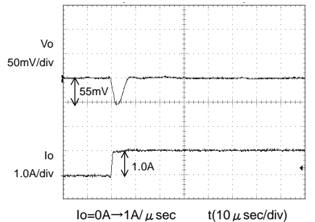
Fig.9 Transient Response (0→1.0A) Co=22 \mu F, Cfb=1000pF
