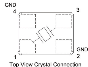
Top View Crystal Connection
