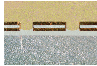
Henkel has the ability to laminate heavy copper up to 5 oz. (175µm) finished on the internal layer utilizing a thicker deposit of HT dielectric.
