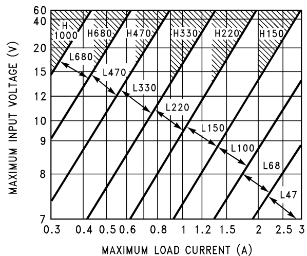
Figure 24. LM2576(HV)-5.0
