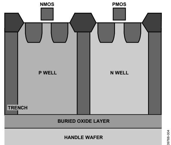
Figure 33. Trench Isolation
