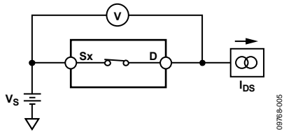
Figure 24. On Resistance
