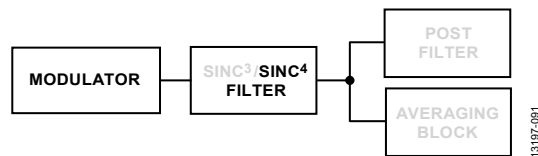
Figure 82. Sinc 4 Filter
