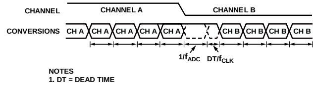
Figure 99. Fast Settling, Sinc 4 + Sinc 1 Filter
