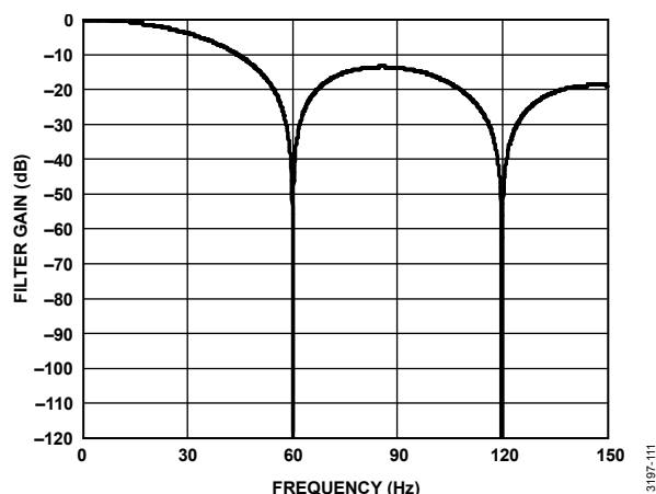
Figure 102. 60 Hz Rejection
