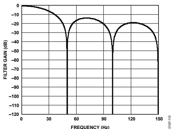
Figure 101. 50 Hz Rejection
