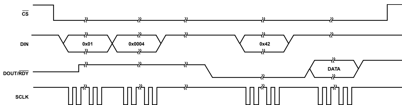
Figure 79. Single Conversion Configuration
