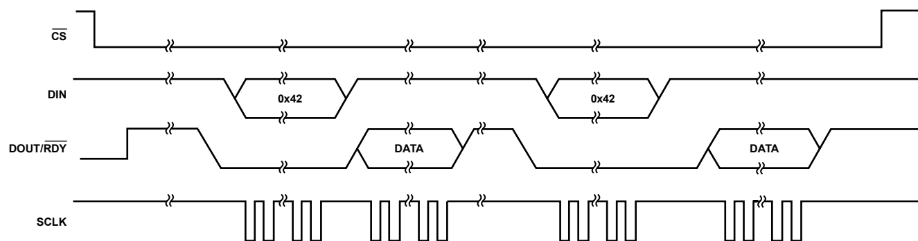
Figure 80. Continuous Conversion Configuration
