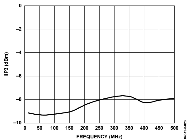
Figure 23. Input IIP3 vs. Frequency ( f_{CLK} = 26\text{ MSPS} )
