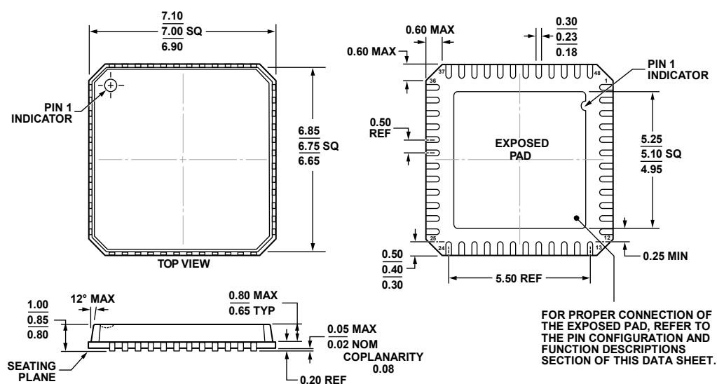
Figure 78. 48-Lead Lead Frame Chip Scale Package [LFCSP] 7 mm × 7 mm Body and 0.85 mm Package Height (CP-48-1)
