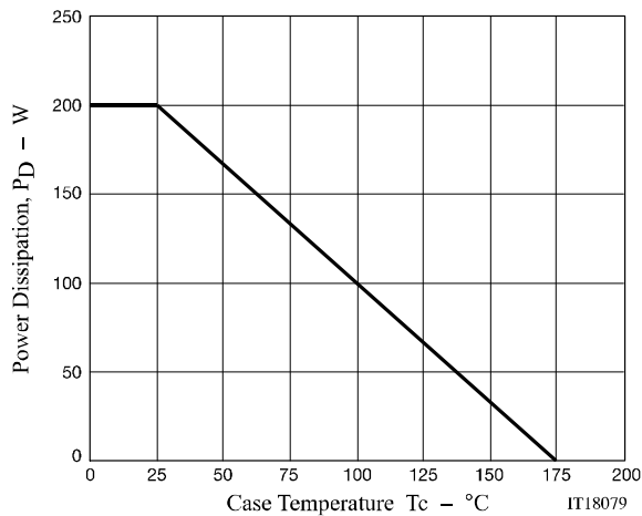
Figure 11. P_D - T_C
