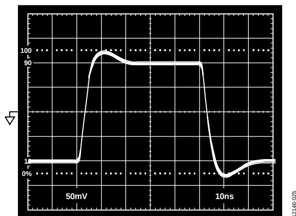
Figure 25. 200 mV Step Response; G = +2 , V_S = \pm 2.5 \text{ V} or \pm 5 \text{ V}
