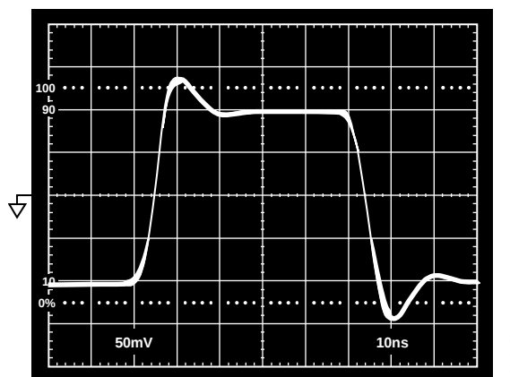
Figure 28. 200 mV Step Response; G = -1 , V_S = \pm 2.5 \text{ V} or \pm 5 \text{ V}
