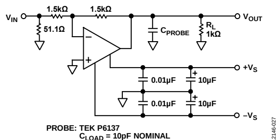
Figure 27. Test Circuit; G = -1 , R_F = R_G = 1.5 \text{ k}\Omega for N-8, R-8, and RJ-5 Packages
