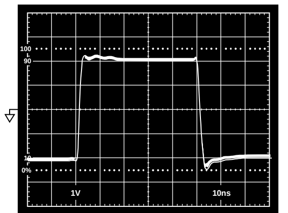
Figure 29. Step Response; G = -1 , V_S = \pm 5 \text{ V}
