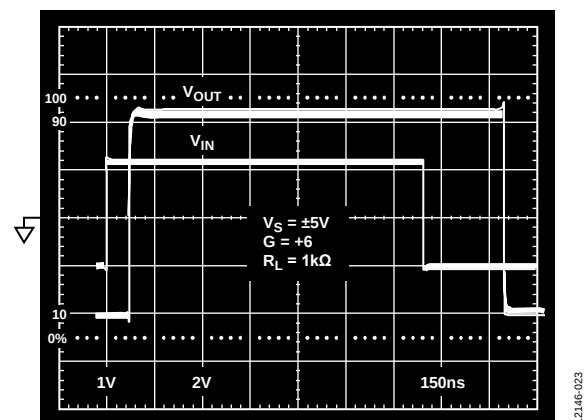
Figure 23. \pm Overdrive Recovery, V_S = \pm 5\text{ V} , V_{IN} = 2\text{ V} Step
