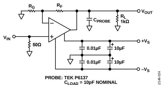
Figure 24. Test Circuit; G = +2 ; R_F = R_G = 3.01 \text{ k}\Omega for N-8 Package; R_F = R_G = 2.49 \text{ k}\Omega for R-8 and RJ-5 Packages
