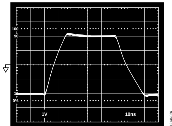
Figure 26. Step Response; G = +2 , V_S = \pm 5 \text{ V}
