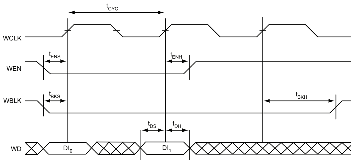
Figure 2-49 • FIFO Write
