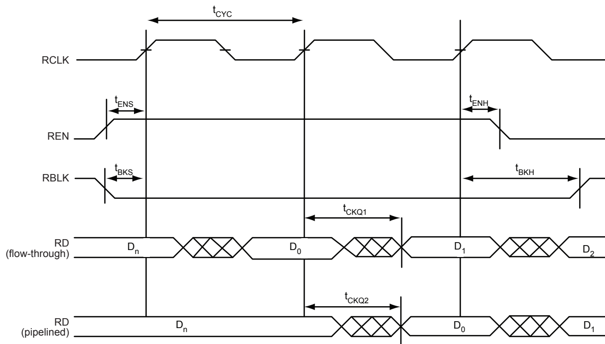
Figure 2-48 • FIFO Read
