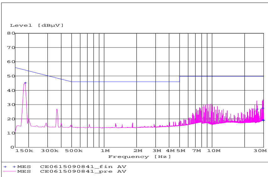
Figure 25. EMC Considerations
