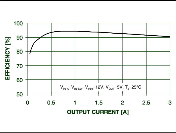
Figure 20. Efficiency vs. output current@ V_{out} = 5\text{ V}
