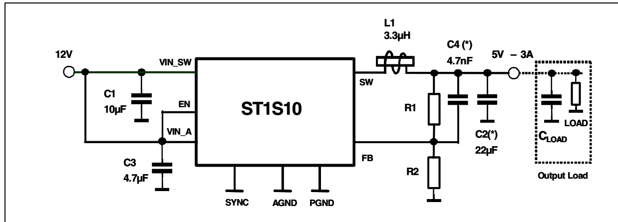
Figure 3. Application schematic for heavy capacitive load
