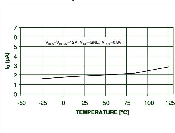
Figure 16. Shutdown mode quiescent current vs. temperature
