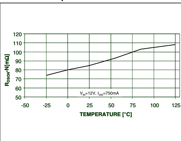
Figure 18. NMOS ON resistance vs. temperature
