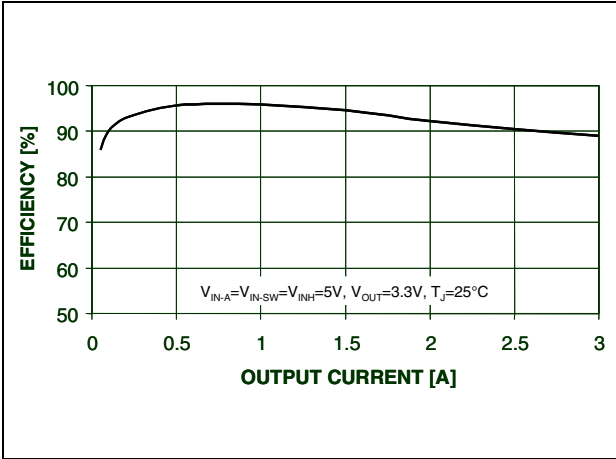
Figure 21. Efficiency vs. output current@ V_{out} = 3.3\text{ V}
