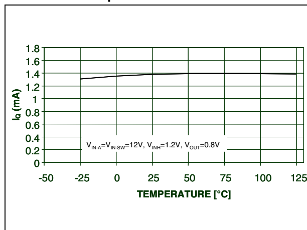
Figure 15. ON mode quiescent current vs. temperature
