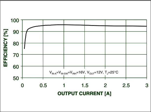
Figure 22. Efficiency vs. output current@ V_{out} = 12\text{ V}
