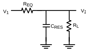
Figure 26. Switched Capacitor Equivalent Circuit
