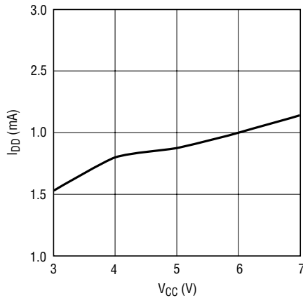
I_{DD} vs V_{CC}
