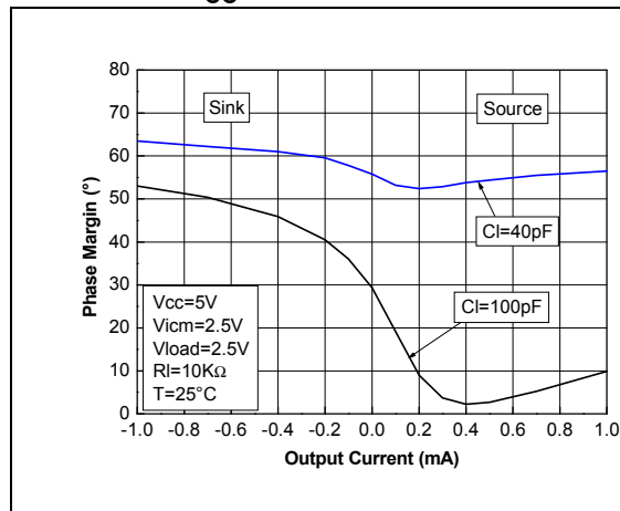
Figure 12. Phase margin vs. output current at V_{CC} = 5 V
