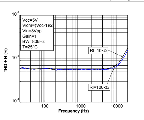
Figure 19. Distortion + noise vs. frequency
