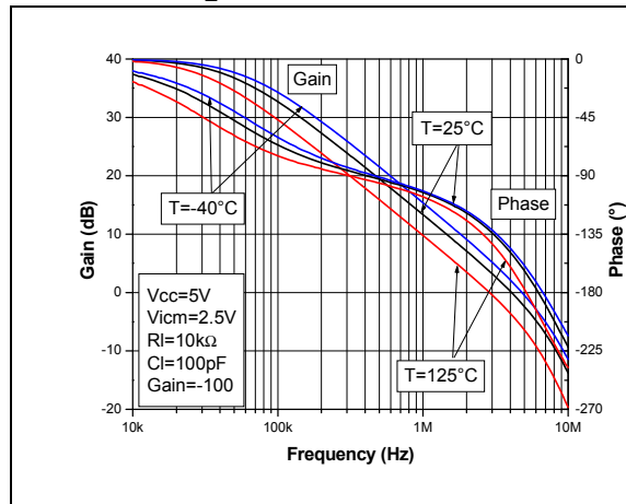
Figure 10. Voltage gain and phase with C_L = 100 pF
