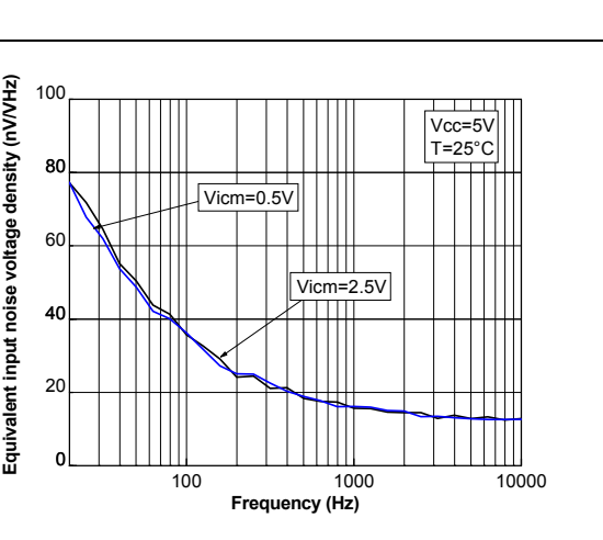
Figure 17. Noise vs. frequency at V_{CC} = 5\text{ V}
