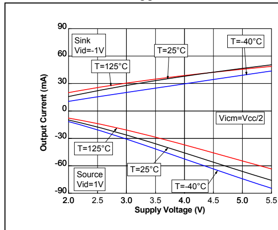
Figure 8. Output current vs. supply voltage at V_{icm} = V_{CC}/2
