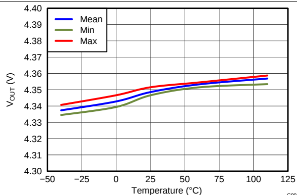
Figure 2. Overtolerance Threshold (OVT) vs. Temperature
