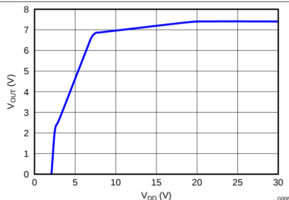
Figure 19. V OUT vs. V DD
