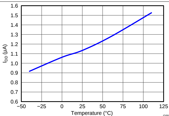
Figure 16. I DD Current Consumption vs. Temperature at V DD = 16 V
