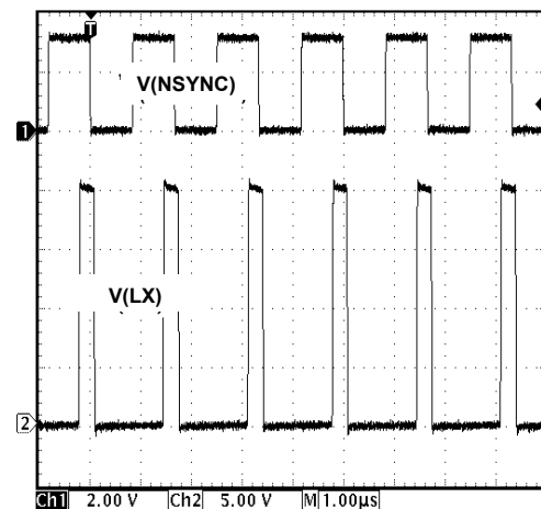
FIGURE 16. LX SYNCHRONIZATION WITH f(SYNC) = 600kHz
