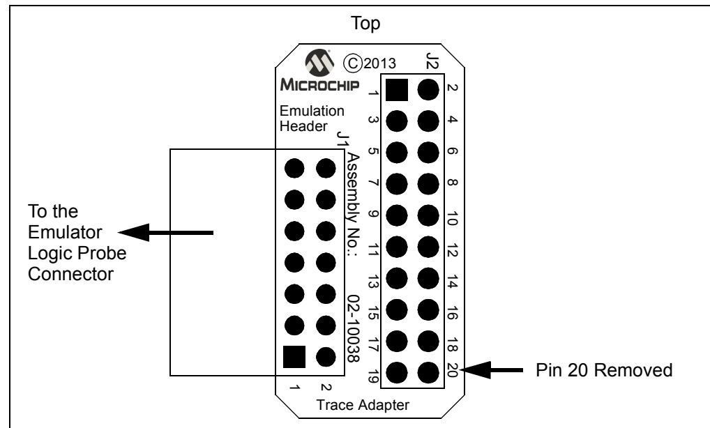
FIGURE 2-4: INTERFACE BOARD
