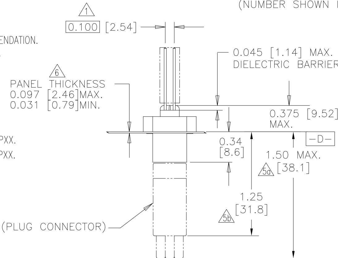
VIEW W-W
