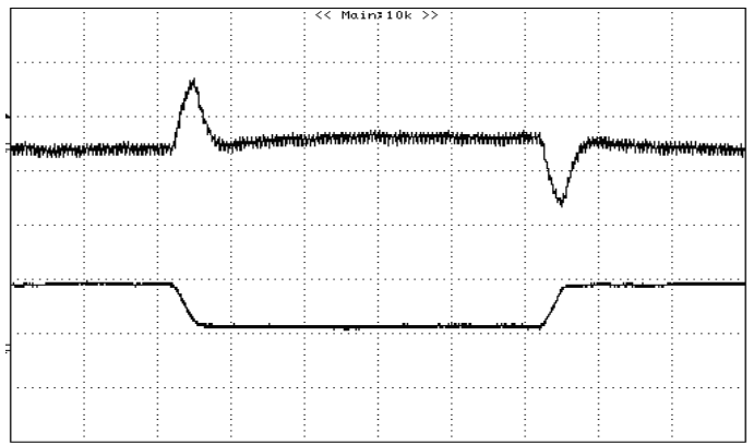
Figure 26: Typical transient response to step load change at 5A/\mu S from 25% to 75% of I_{o, max} at 12Vin, 5V out (Cout = 1uF ceramic, 10uF tantalum) Top:100mV/div, 50uS/div, Bottom: 20A/div, 50uS/div
