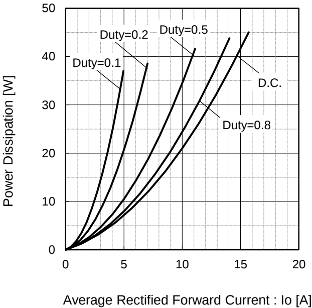
Fig.8 Io-Pf Characteristics
