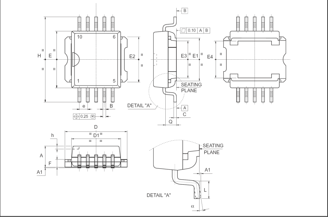
Figure 10. Package dimension
